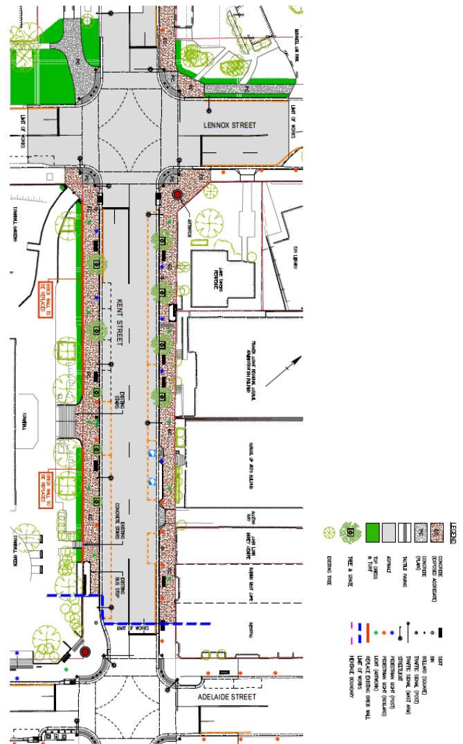
Layout Plan—Kent Street
