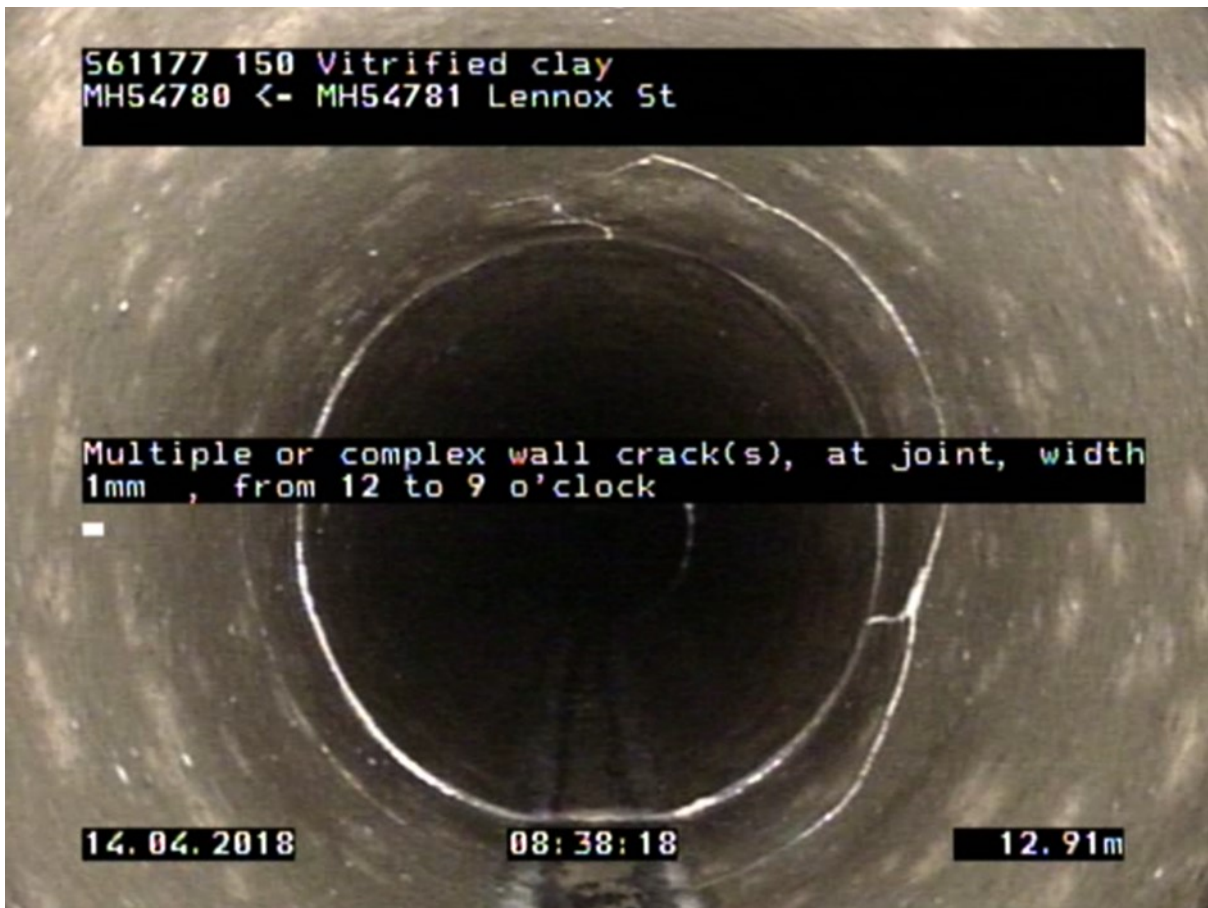
Fig. 1 Sewer Main in Lennox prior to rehabilitation program
