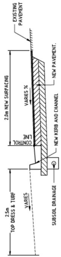
TYPICAL SECTION (BOTH SIDES) NOT TO SCALE
