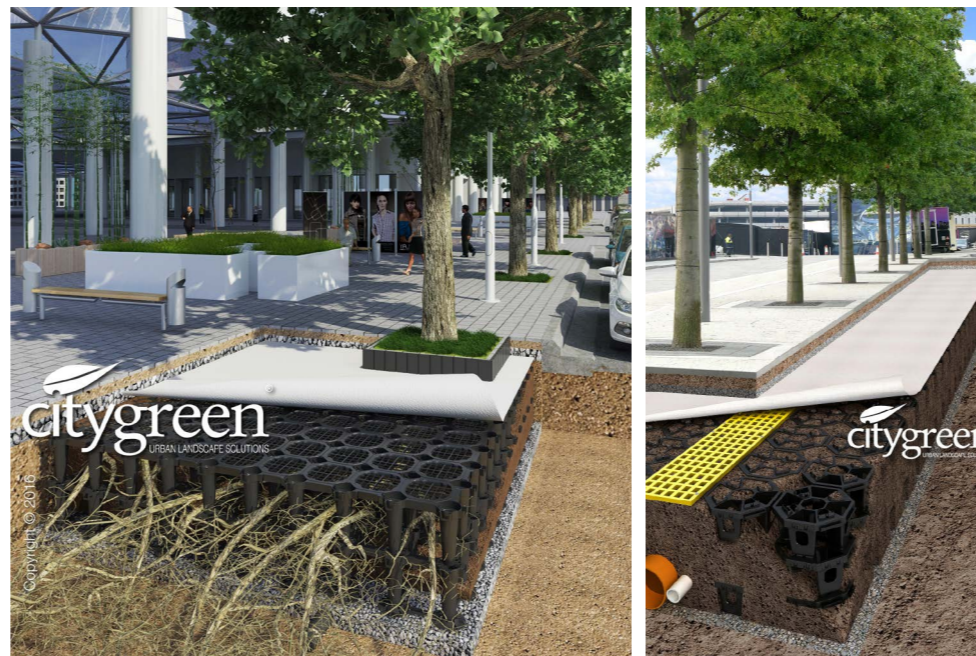
FIGURE 9 : Example of engineered soil cell installed under roadway and footpath pavement. Images Courtesy of Citygreen.
