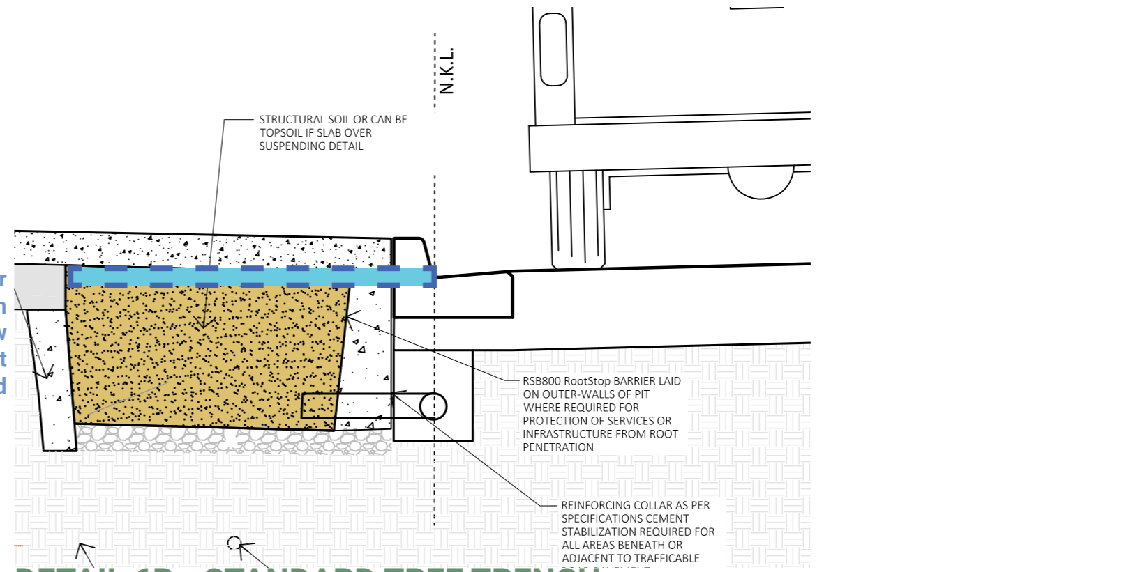
DETAIL 6B - STANDARD TREE TRENCH
