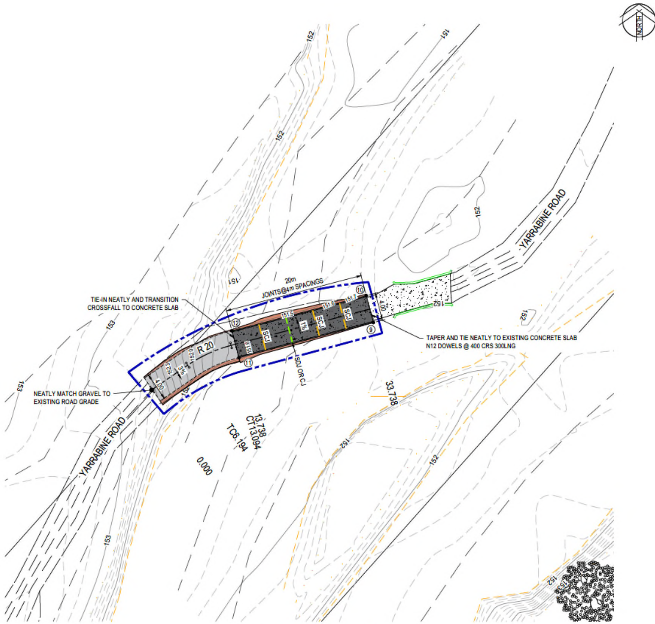
LAYOUT PLAN - CROSSING 3 SCALE 1:200
