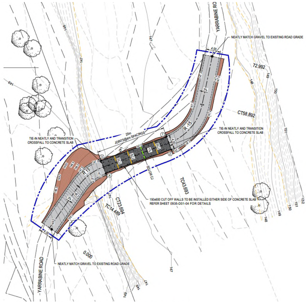
LAYOUT PLAN - CROSSING 1 SCALE 1:200
