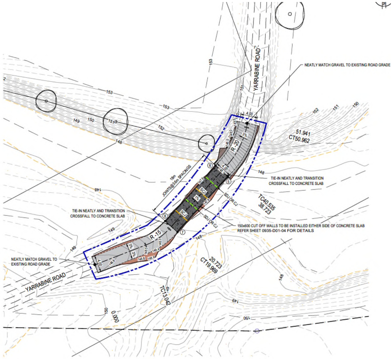
LAYOUT PLAN - CROSSING 2 SCALE 1:200
