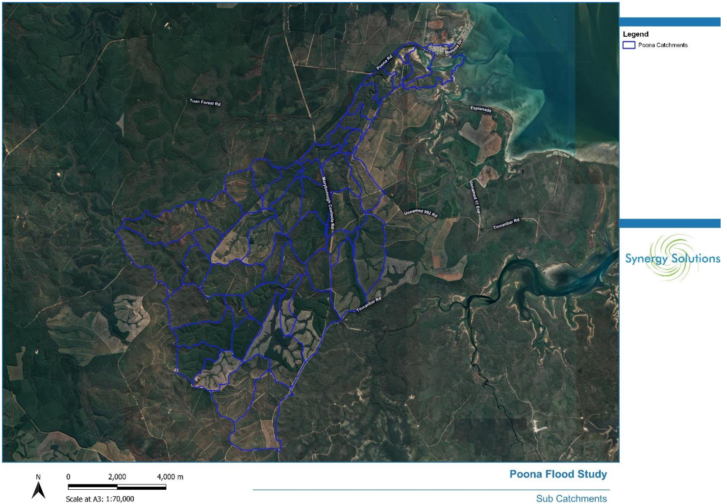
Figure 5-1 Sub Catchments
