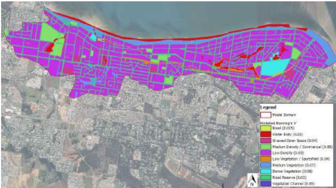
Figure 2-6 Modelled Roughness
